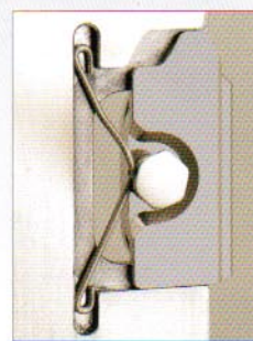
Detail: interchangeable tooth.
